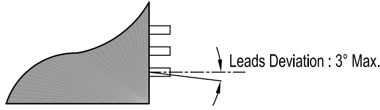
DETAIL A
